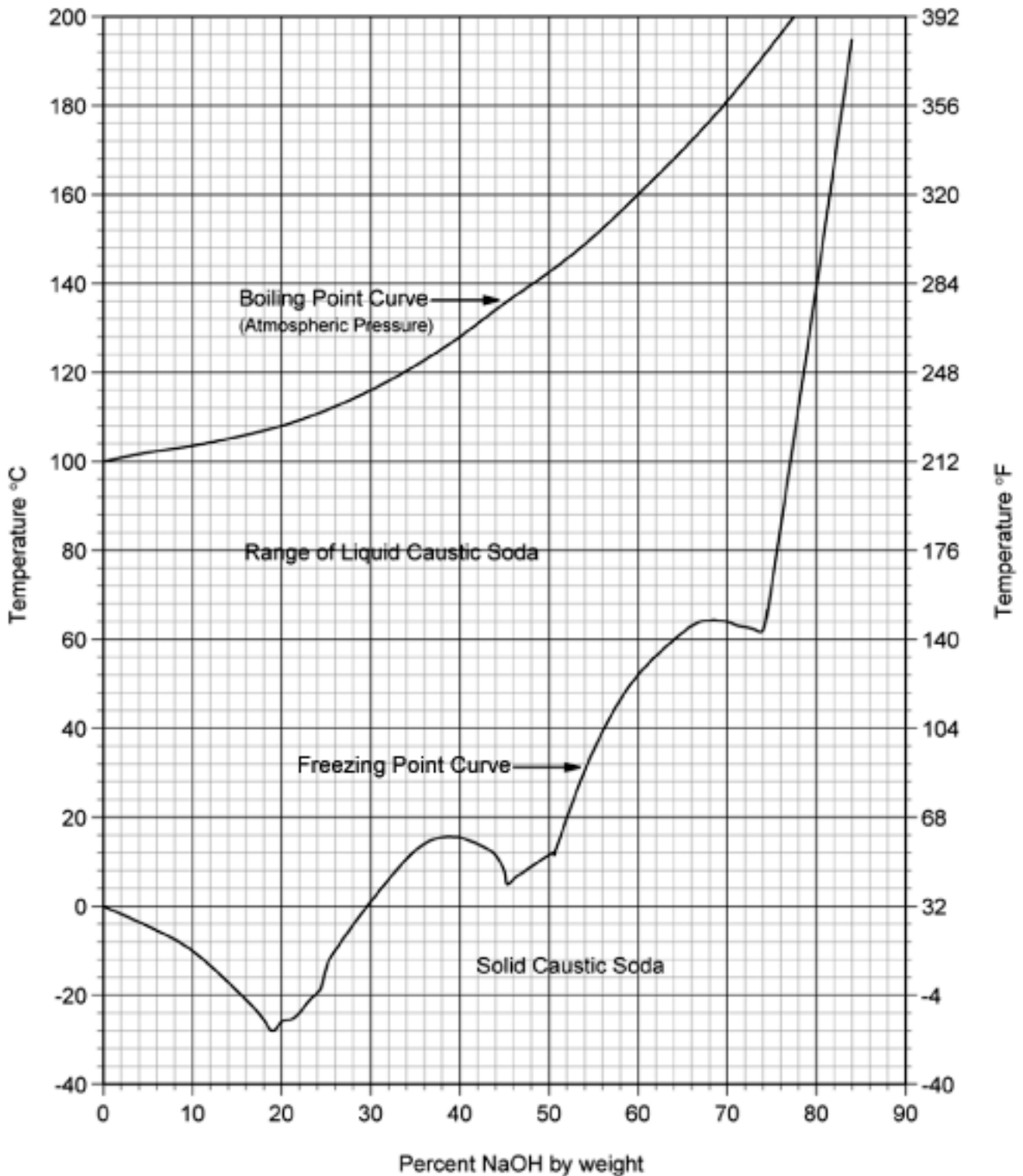
Graph 1 Boiling and Freezing Temperatures of Aqueous Caustic Soda Solutions
